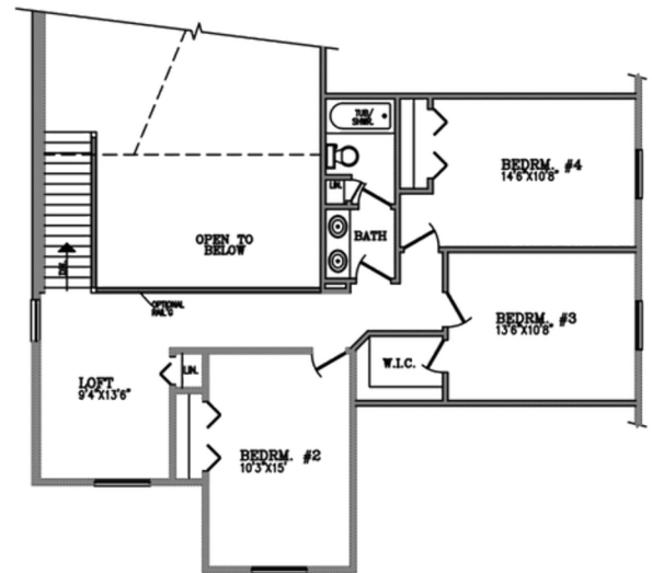
SECOND FLOOR PLAN 4 Bedroom Option
